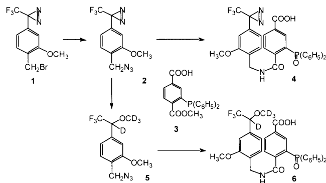
Fig. 1. Synthesis of the Alkylazide Derivative of the (3-Trifluoromethyl) Phenyldiazirine Derivative and Its Application to the Staudinger–Bertozzi Ligation
